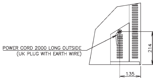
VIEW A
